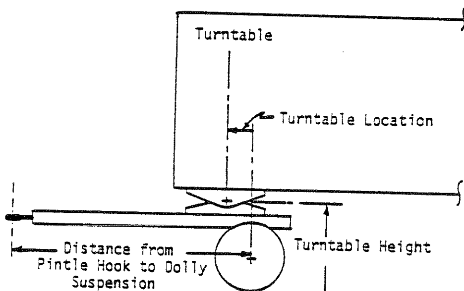
Converter Dolly
