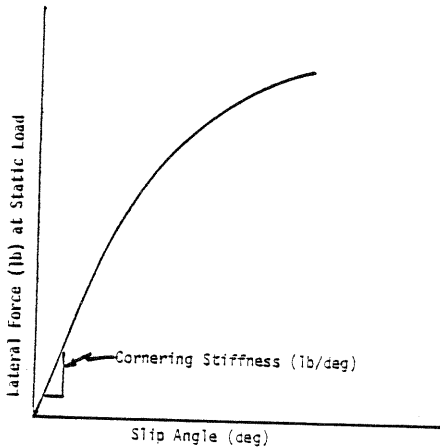
Figure 7. Definition of cornering stiffness parameter.
