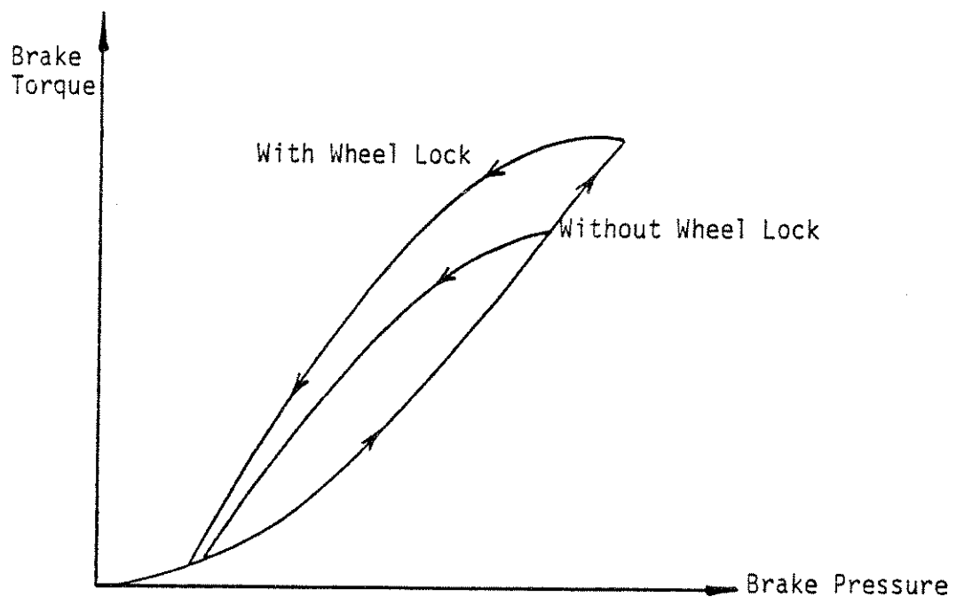
Figure I.6-1. Brake torque-pressure hysteresis characteristic.
