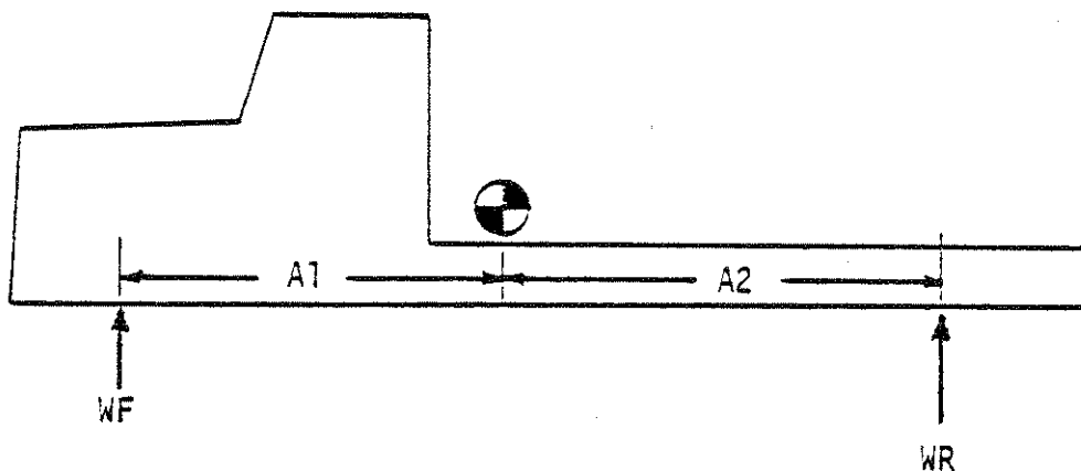
Schematic diagram of sprung mass
