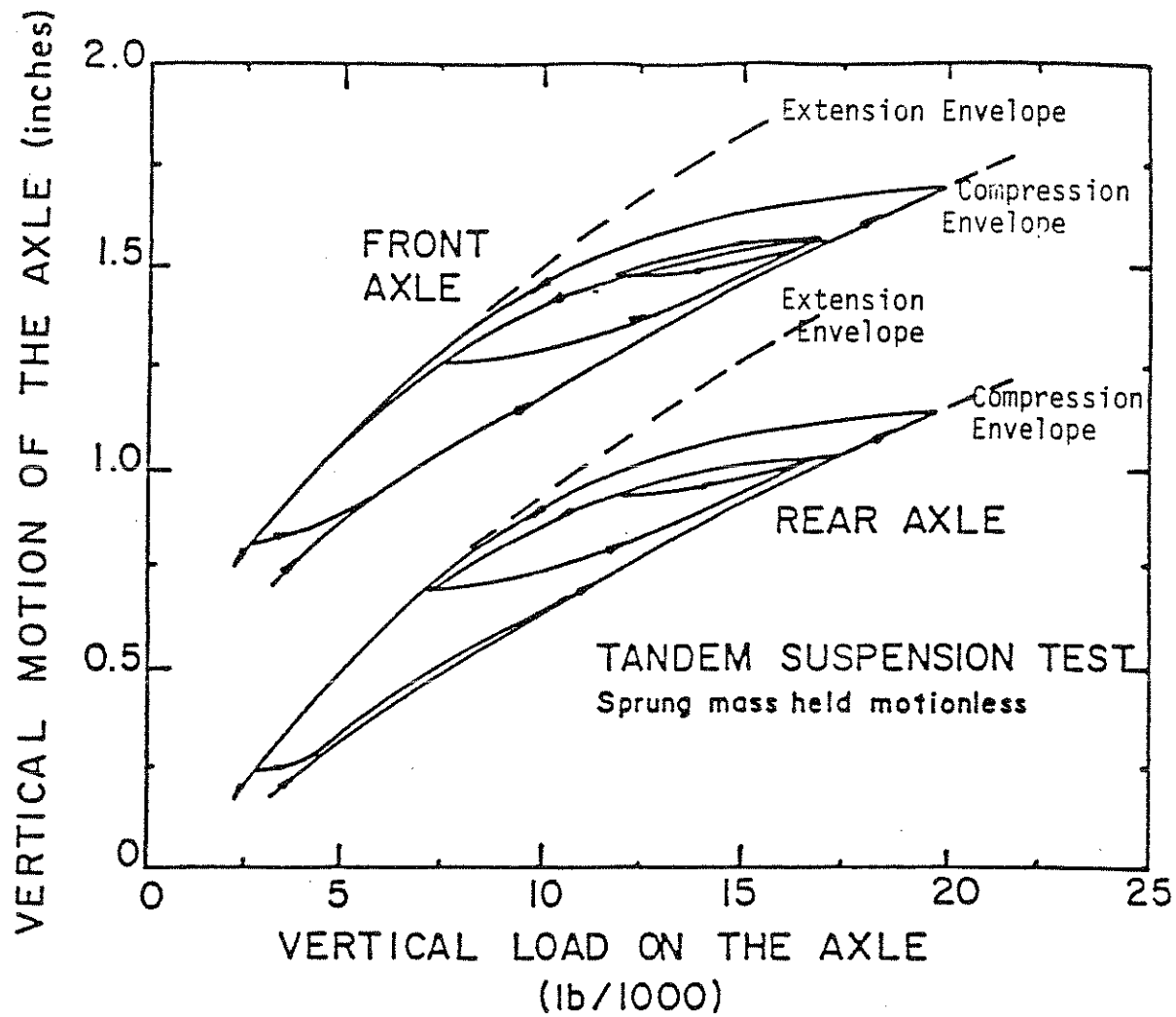
Figure I.3-1. Rear tandem suspension force-deflection measurement.
