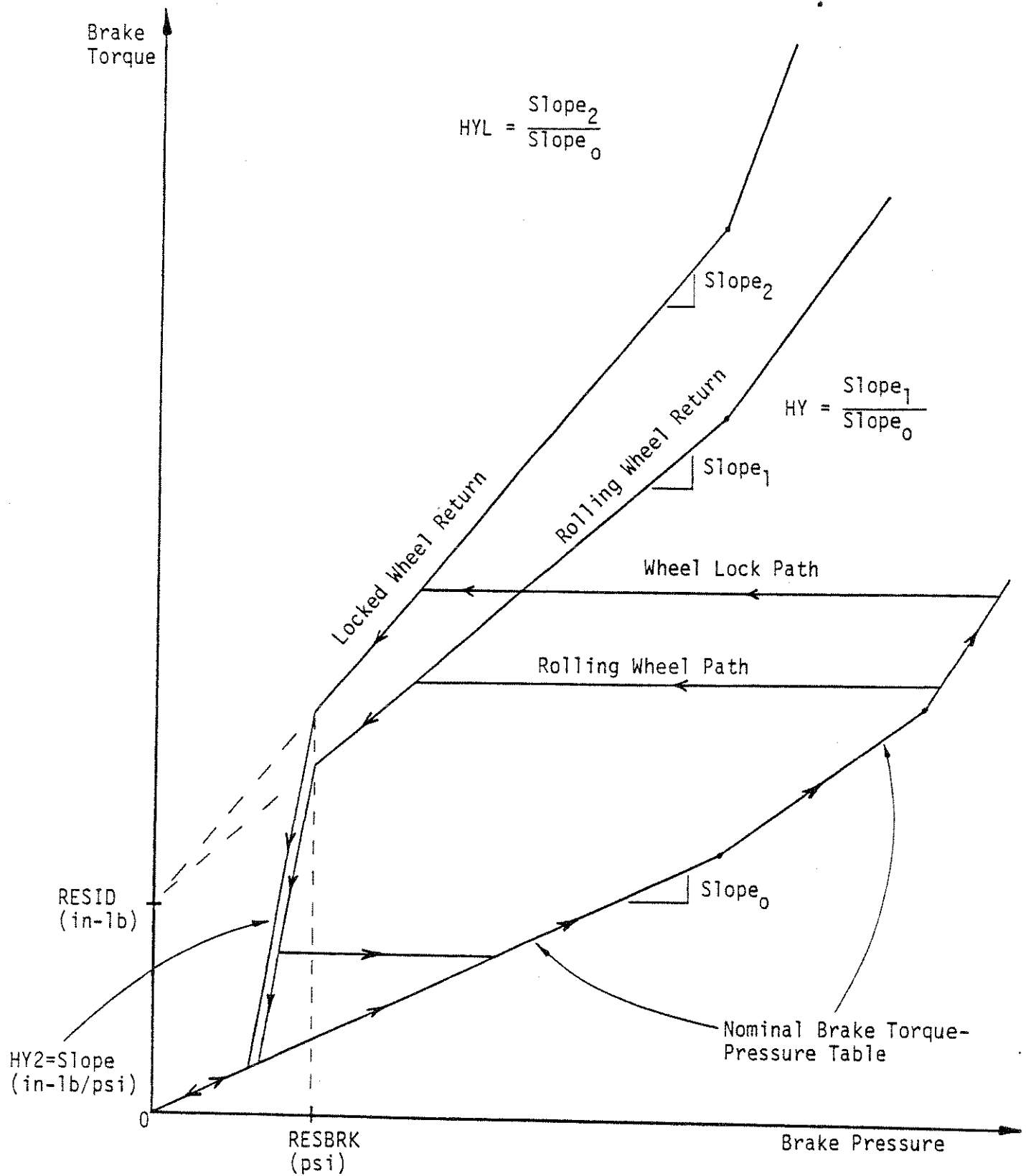
Figure I.6-2. Brake hysteresis algorithm and definition of input parameters: HY, HY2, RESBRK, RESID, and HYL.
